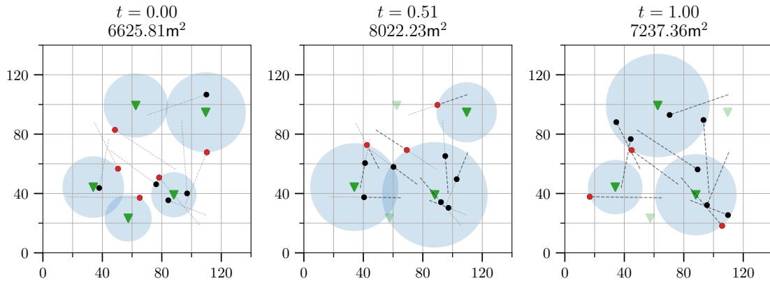
Figure 1: An optimal solution for 10 moving points and 5 stations depicted as triangles. Our algorithm can find a solution over time, that uses at most 8022.23\text{m}^2 of area over the whole time interval. This solution is matched by a lower-bound computed by solving the static DC problem at this time step.
